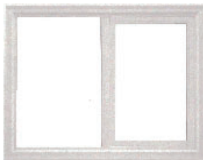
Sliding Window
